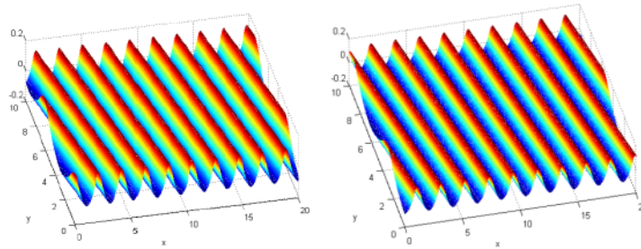
Figure 2. Wave profile at t = 0 (left) and t = 10 (right) with monochromatic as signal input.
