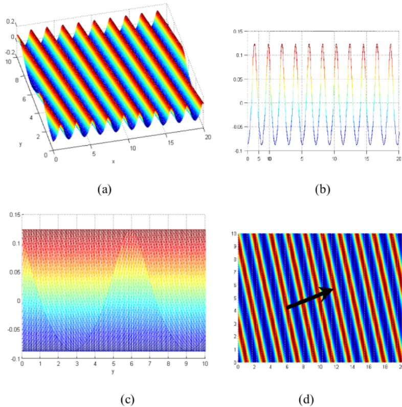
Figure 4. Wave profile at t = 0 (a), looked from x side (b) and y side (c), the direction of wave propagation (d).
