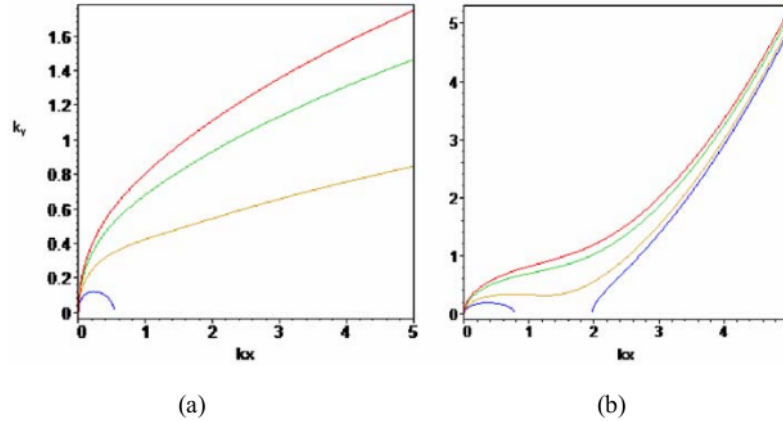
Figure 1. The relation between wave numbers k_x and k_y for KP_{AB} (a) and KP type with KdV (b).
