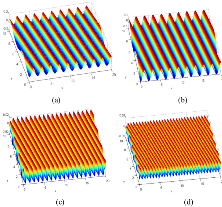
Figure 3. The profile of wave at t = 0 (a) with the first (b), second (c) and third (d) order contribution of the solution of KP.
