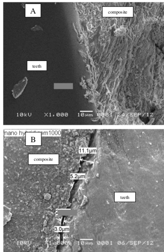
FIG. 2 INTERACTION BETWEEN TEETH AND (A) METAKAOLIN-ZIRCONIA-APATITE NANOCOMPOSITE, (B) COMMERCIAL NANOHYBRID COMPOSITE
