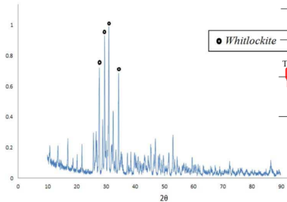
FIG. 1 DIFFRACTOGRAM OF THE APATITE
