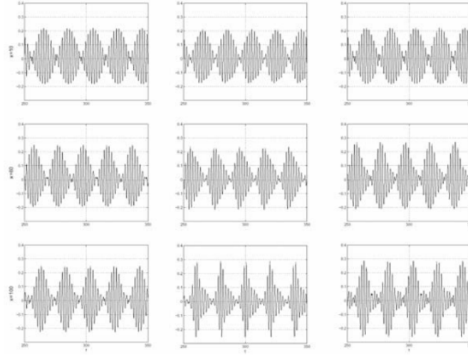
Figure 7. The bi-chromatic signals computed with third order asymptotic of KdV (left) and numerical simulation of AB (mid) and third order asymptotic of AB(right) at x = 10, 60, 100\text{m} .
