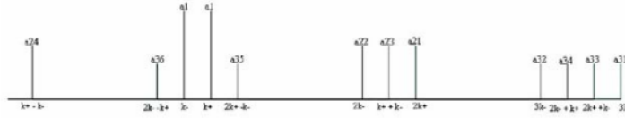
Figure 1. Nonlinear mode generation in second and third order from the two basic wave numbers in the bi-chromatic wave.
