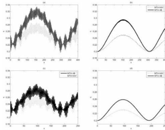
Figure 9. MTA curve for different parameter v , (a) v = 0.1575[1/s] (c) v = 0.2[1/s] with second order solution and (b) v = 0.1575[1/s] (d) v = 0.2[1/s] without second order solution for AB (continues line) and KdV (dot line), for amplitude a = 0.05[m] and frequency \bar{\omega} = 3.1495[1/s] .
