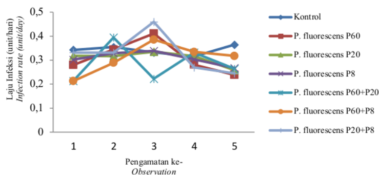
Gambar 1. Perkembangan laju infeksi penyakit antraknosa selama pengamatan Figure 1. Development of the disease infection rate during observation
