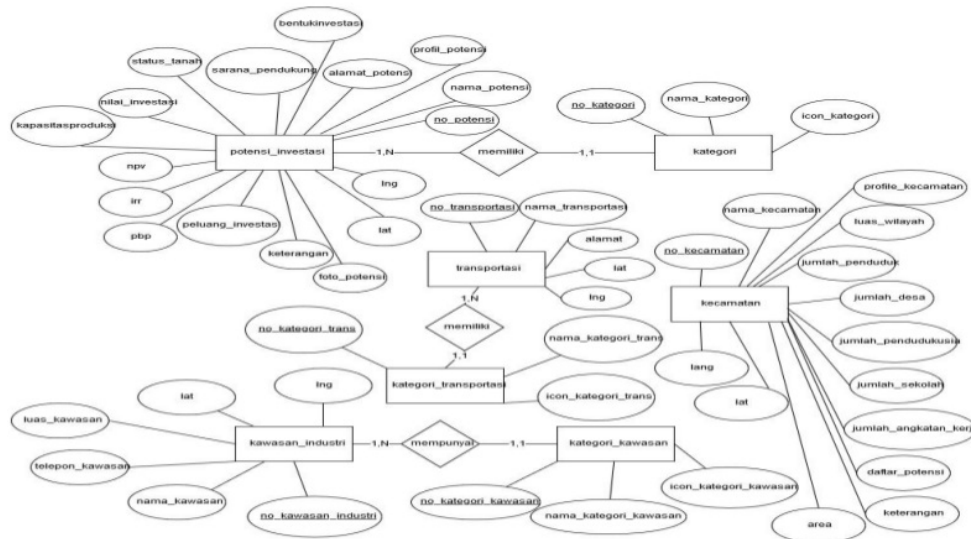
Gambar-7 Entity Relationship Diagram SIG
