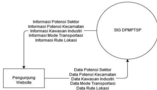
Gambar-5 Data Flow Diagram Level 0
