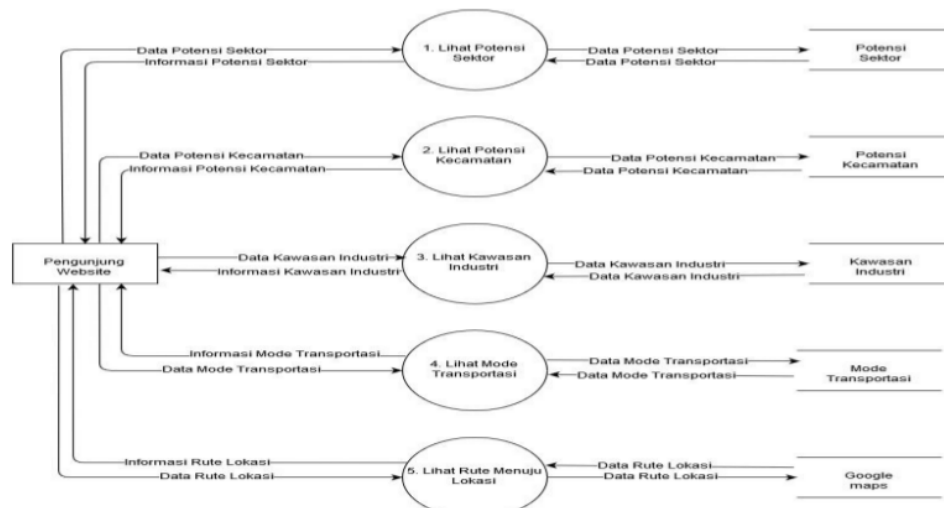
Gambar-6 Data Flow Diagram Level 1
