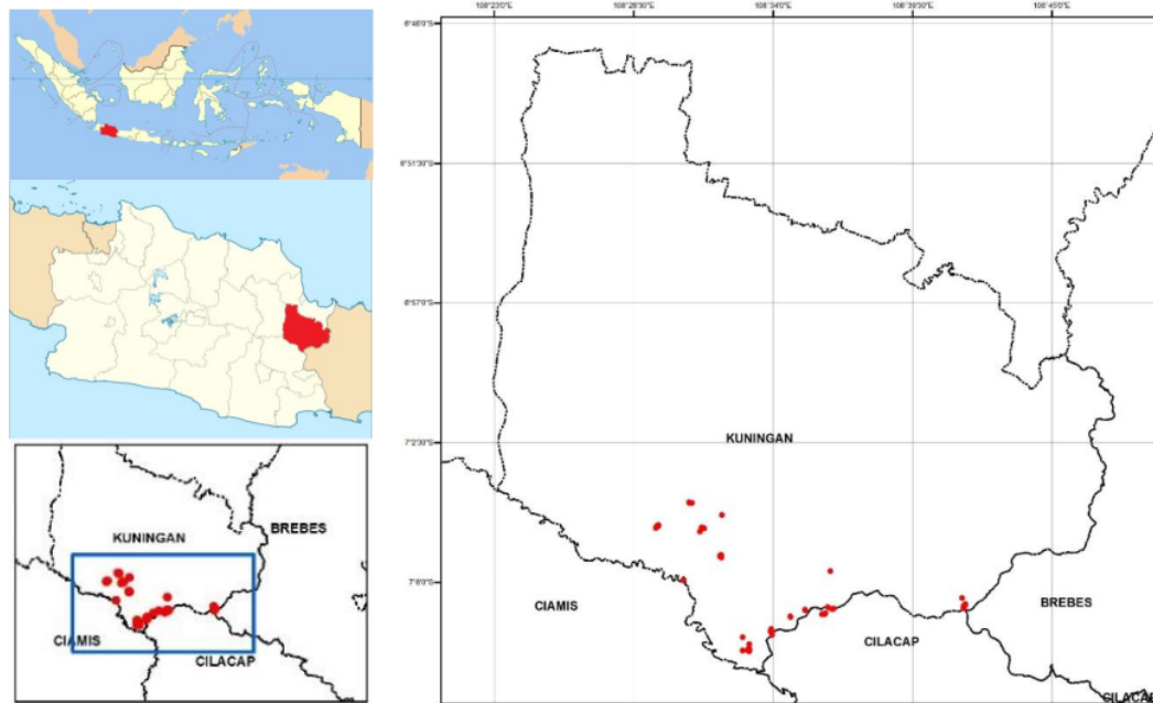
Figure 1. Study area and seventeen sampling sites of Goniothalamus macrophyllus in Bukit Pembarisan, Kuningan District, West Java, Indonesia 2
