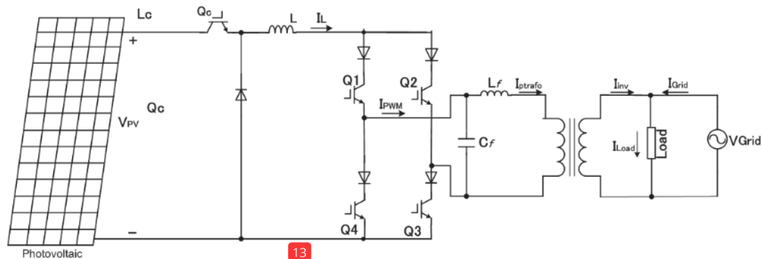
FIGURE 2. Proposed grid connected photovoltaic system
