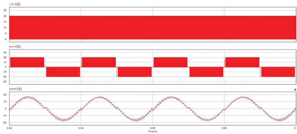
FIGURE 5. Current waveform during grid connected operation.
