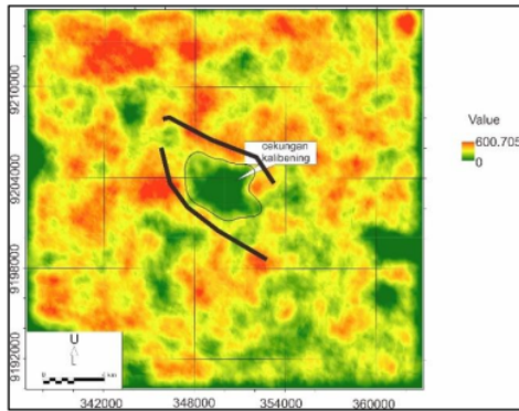
Gambar 5. Peta Fault Fracture Density (FFD).
