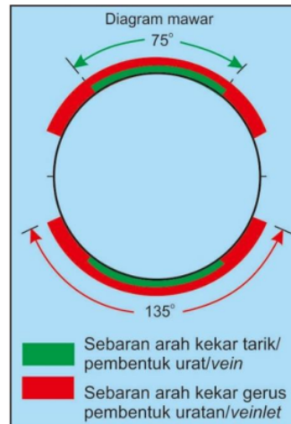
Gambar 8. Rentang arah urat dan uratan kuarsa hasil gaya utara-selatan (Singhal and Gupta, 2010)
