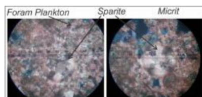
Figure 12. Planktonic Foraminifera Appearance (Facies at Location J)
