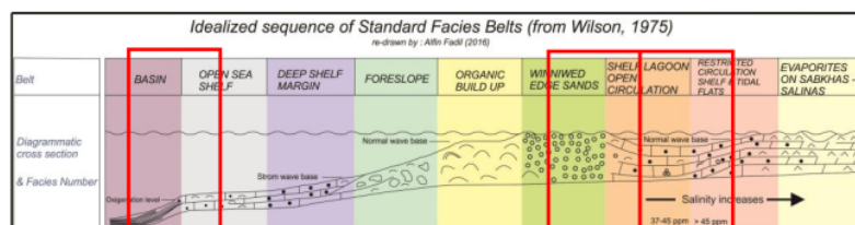
Figure 13. Facies environment according to Wilson (1975)
