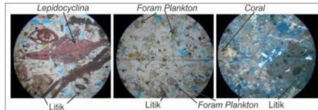
Figure 9. The appearance of planktonic Foraminifera - Lepidocyclina at Location G.
