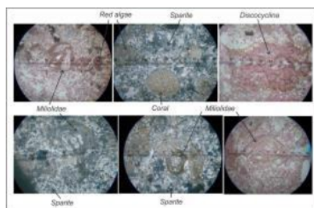
Figure 3. Miliolid appearance (Facies at Location A)
