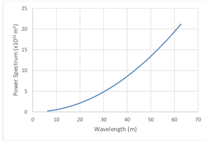
Figure 2. Plot Power Spectrum of Scalar Perturbation of Starobinsky's Inflation Model to The Wavelength Perturbation.
