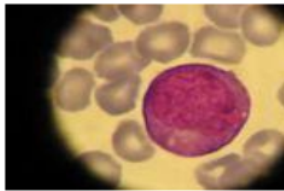
Figure 1. Blood cell
