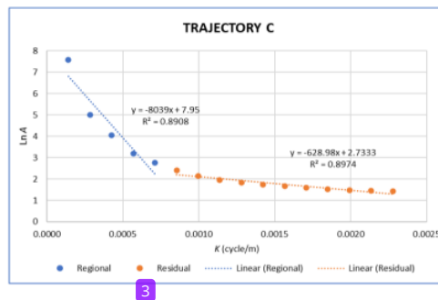
Figure 10. The result of power spectrum analysis of the CBA data on trajectory C which have been spread on a horizontal surface.
