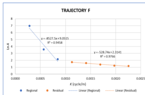
Figure 13. The result of power spectrum analysis of the CBA data on trajectory F which have been spread on a horizontal surface.
