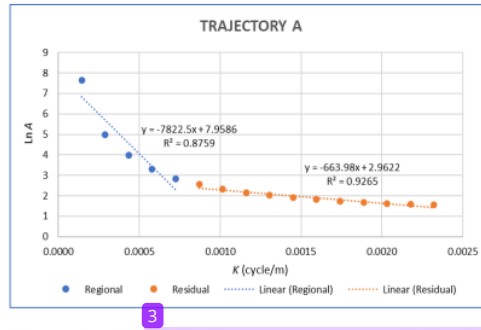
Figure 8. The result of power spectrum analysis of the CBA data on trajectory A which have been spread on a horizontal surface.
