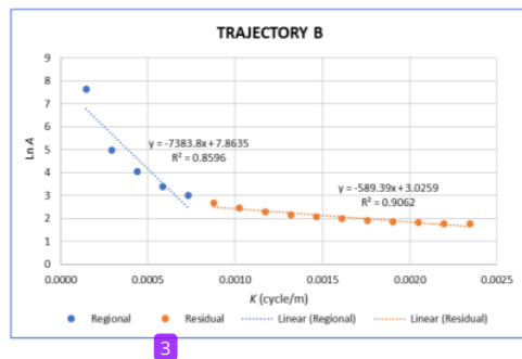
Figure 9. The result of power spectrum analysis of the CBA data on trajectory B which have been spread on a horizontal surface.
