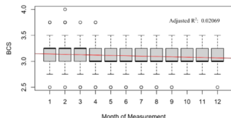
Figure 3. Regression of BCS on month of measurement
