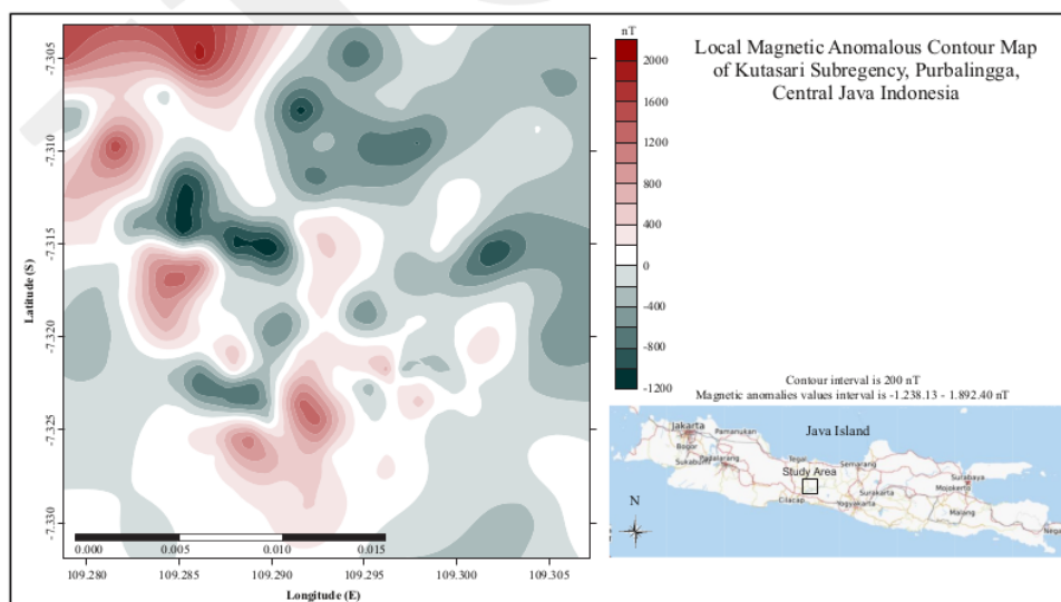
Figure 4. Local magnetic anomalous contour map of the studied area, where these data are distributed on the average topographic height of 438.04 m.
