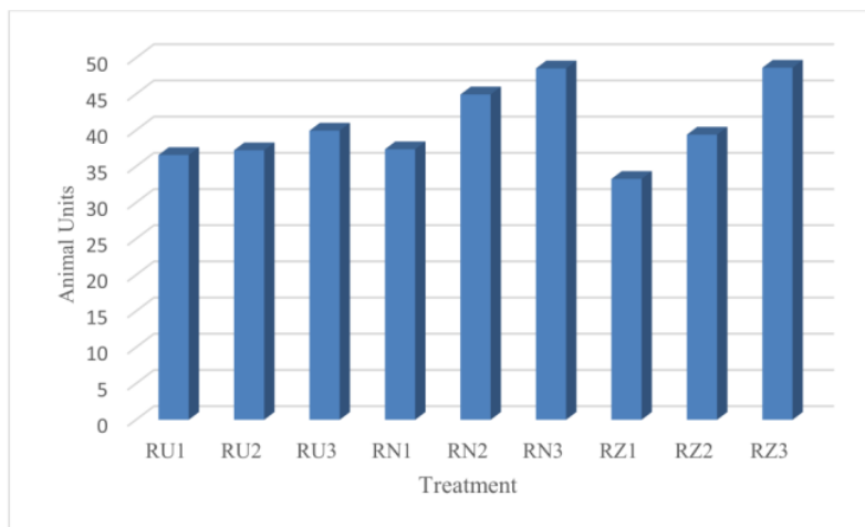
Figure 4. Diagram of the effect of dairy cow manure enriched with various types and levels of inorganic fertilizers on the carrying capacity of King grass. Note. please add the treatment's description.
