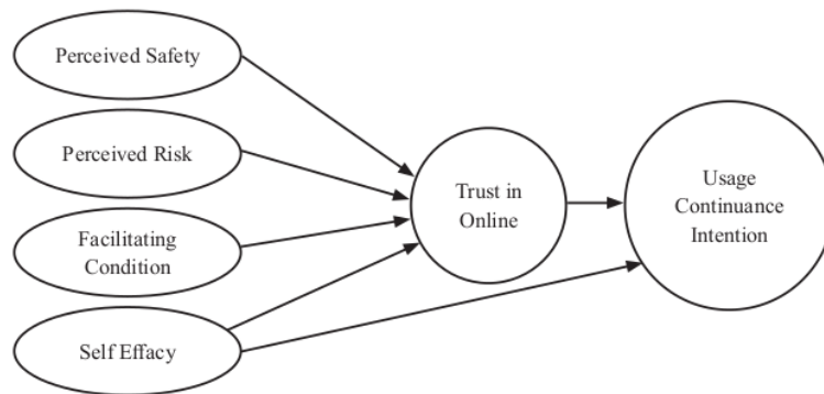
Figure 1. Research Framework
