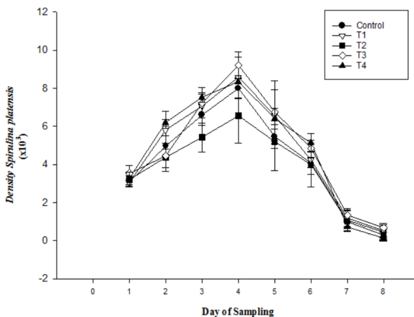
Figure 1. Population density of S. platensis during 8 days of cultivation. The growth media consisted of 3 L diluted (2:1) tofu wastewater at pH 9 and 27°C to 29°C, containing various amounts of urea: 0 g (control), 10 g (T1), 20 g (T2), 30 g (T3), or 40 g (T4) (n = 3 replicates ; data shown mean \pm SD)
