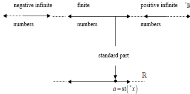
Figure 3.1 Hyperreal Numbers Set
