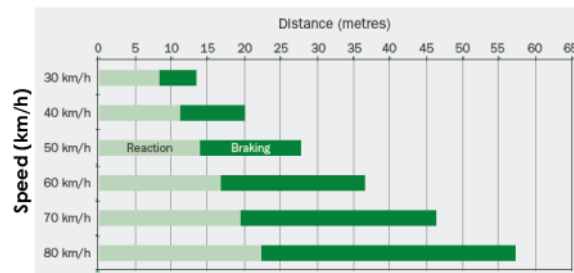
Figure 2 Illustration stopping distance in an emergency braking [19]
