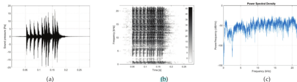
Fig. 2. Sound characteristics of raps; (a) waveform; (b) spectrogram; and (c) PSD
