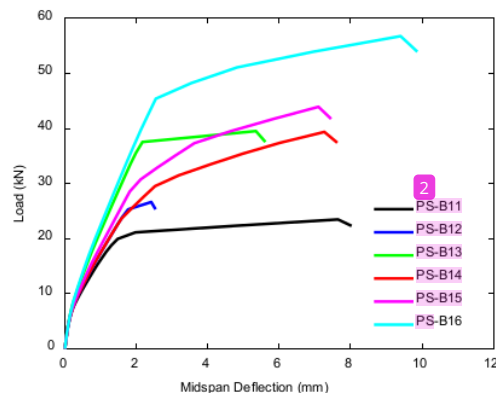
Fig. 9. Impact of steel reinforcement ratio on the beams' performance
