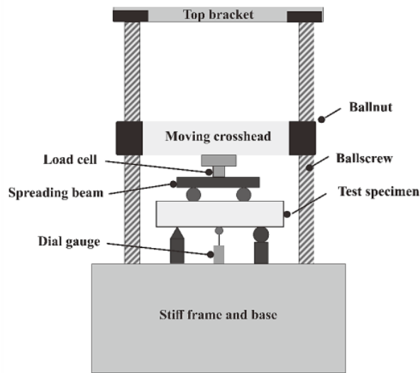
Fig. 2. Experimental setup.
