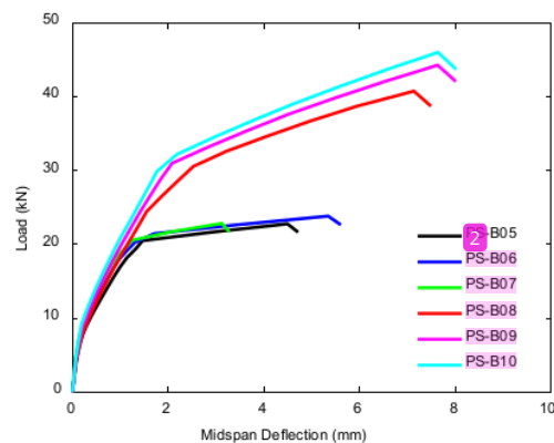
Fig. 8. Impact of compressive strength over beams' performance.
