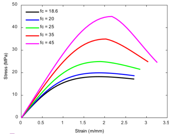
Fig. 3. Compression stress versus strain curve for concrete.
