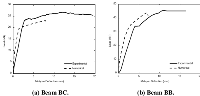
Fig. 5. Comparison of experimental and predicted load-deflection curves.
