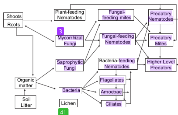
Fig. 2. Summary of the soil food web model used to interpret the data.
