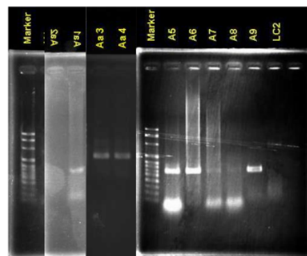
Figure 2. Visualization of PCR products from Aedes albopictus tested for Wolbachia (from 10 specimens tests, there are 6 samples (Ae 2, 3, 4, 5, 6, and 9) specimens are positive for Wolbachia )
