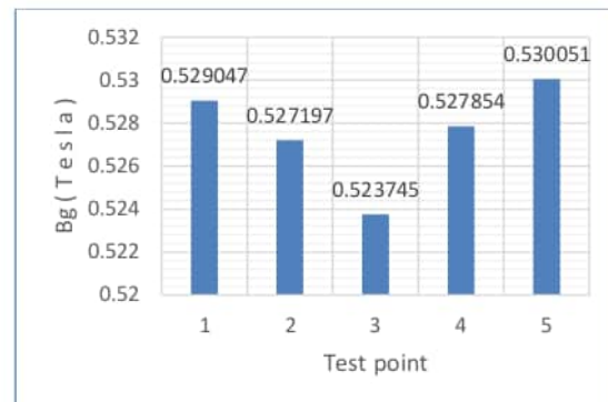
Figure 9 Graph of GSMPFR testing with AWG 14
