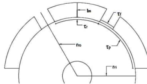
Figure 3 GSMFR rotor dimensions.
