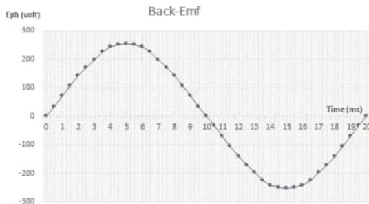
Figure 11 Back-Emf waveform
