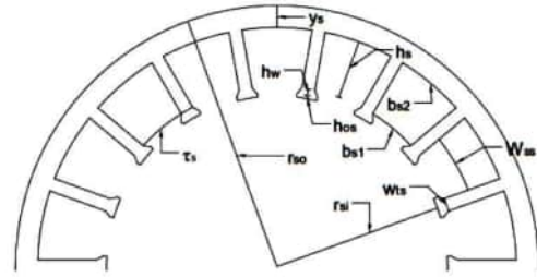
Figure 4 Stator GSPFR specification
