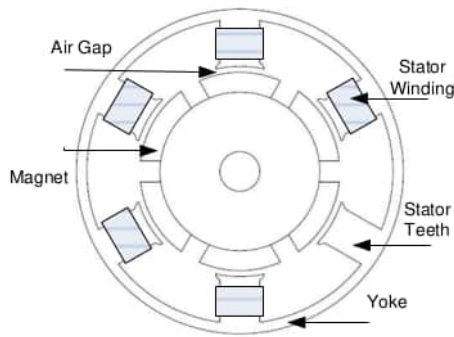
Figure 1 Permanent magnet generator of radial flux
