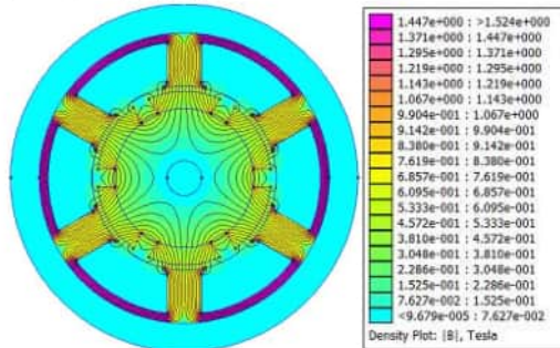
Figure 7 Simulation of magnetic flux density generator design
