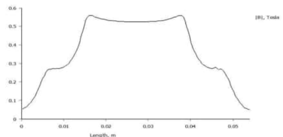
Figure 10 Waveform of air gap flux density distribution
