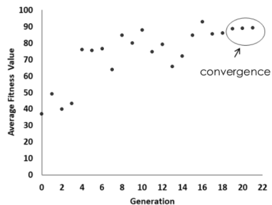
Figure 4 Relation of the increase in generation to the fitness value
