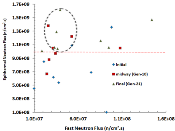
Figure 6 Value of fast neutron flux that accompany epithermal neutron flux in early, middle and late generation
