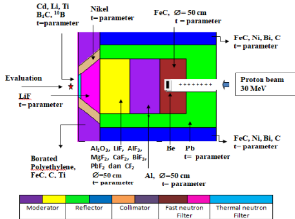
Figure 1 Configuration of double layer BSA
