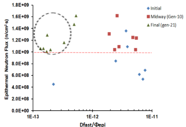
Figure 8 Effect of generation change on the ratio between fast neutron dose rate and epithermal neutron flux in early, middle and late generations
