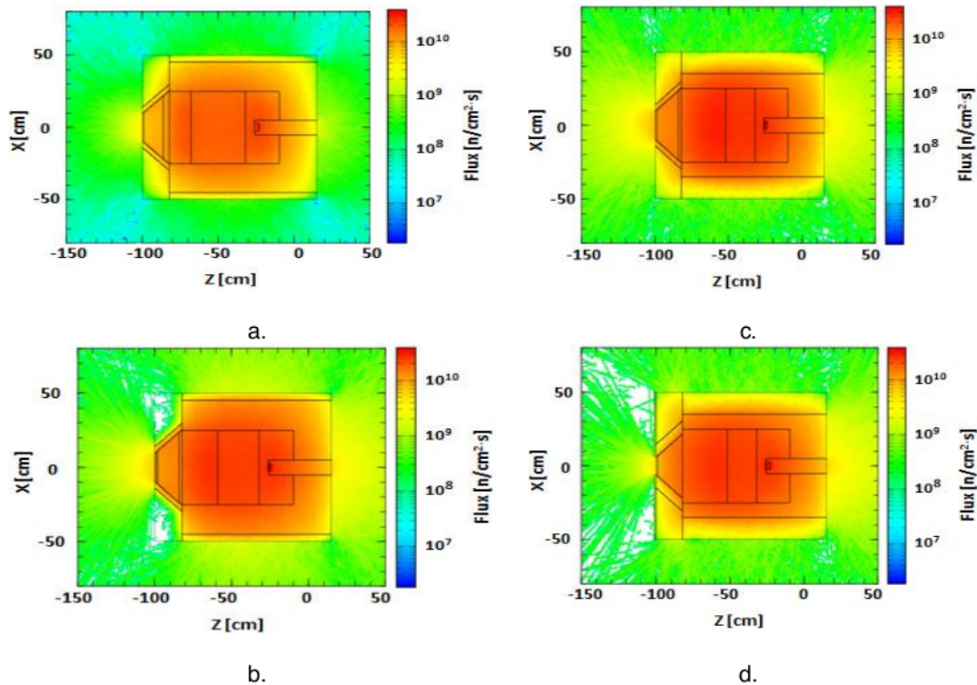
Figure 10 Distribution of epithermal neutron flux in double layer BSA a. K3, b. K4, c.K6, d.K8
