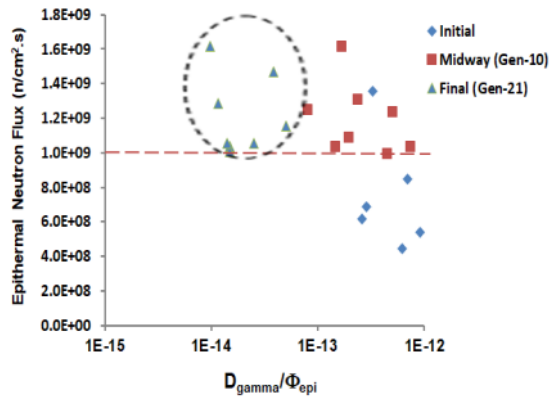
Figure 9 Effect of generation change on the ratio between gamma dose rate and epithermal neutron flux in early, middle and late generations
