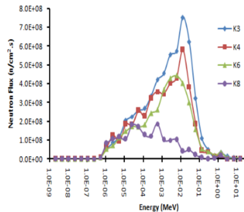
Figure 11 Spectrum of neutron flux produced by DLBSA a. K3, b. K4, c.K6, d.K8
