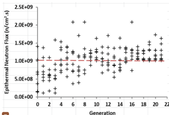
Figure 5 Effect of generation change on epithermal neutron flux
