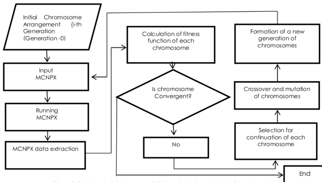
Figure 2 Flowchart of simultaneous DLBSA optimization using the GA method
