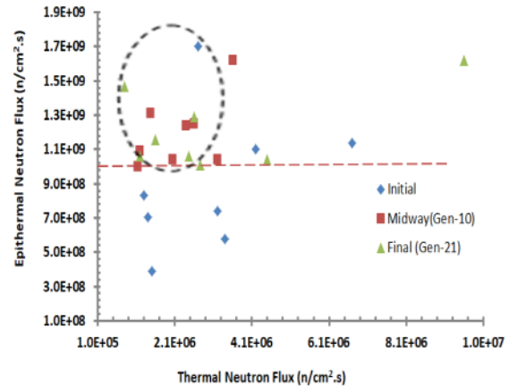
Figure 7 Value of thermal neutron flux accompanying epithermal neutron flux in early, middle and late generations
