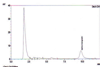
Figure 2. Chromatogram of \alpha -mangostin in the oral solution
