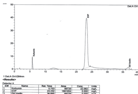
Figure 5. The characterization result by HPLC
