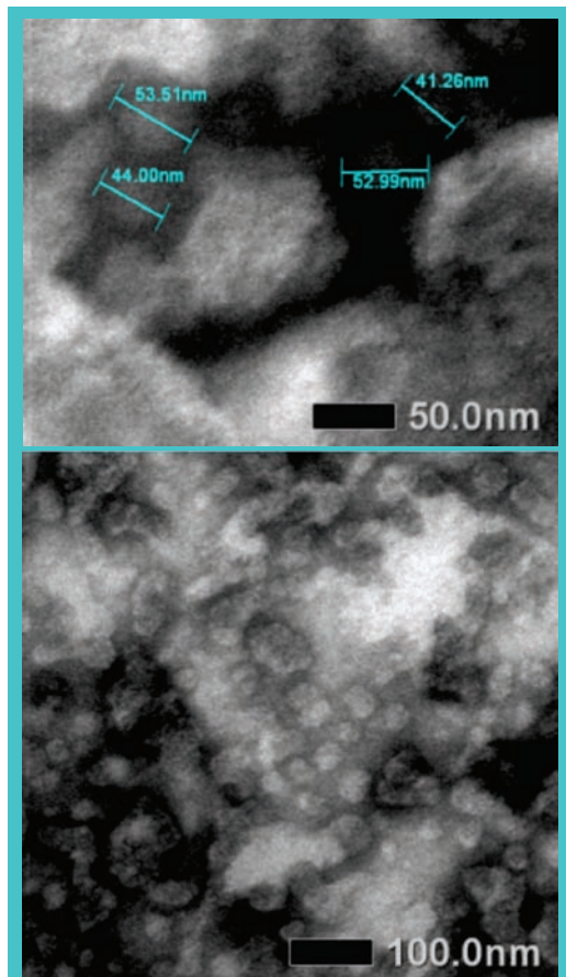
Fig 1. Morfology of SLN-alpha tocopheryl acetate measured by TEM
