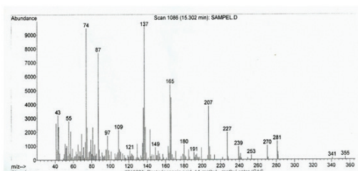
Figure 3. The characterization result by Gas Chromatography-Mass Spectrometry
