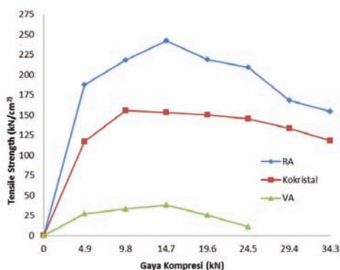
Figure 3 Compressibility Curve
