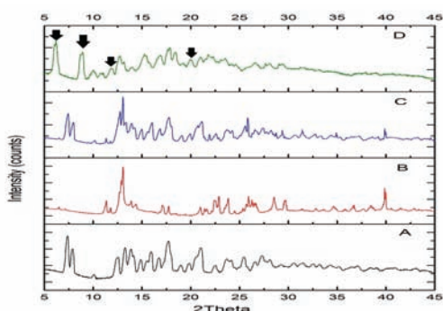
Figure 3 Powder Diffractogram A) RA B) VA C) PM D) RA-VA
