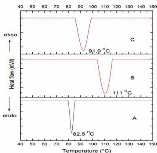
Figure 2 Thermogram DSC A) VA, B) RA C) RA-VA
