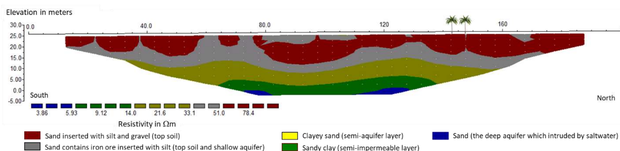
Figure 12. The 2D-hydrogeological profile contour of sub-surface rocks on the WP-03 trajectory
