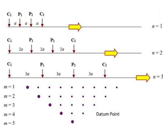
Figure 3. Sketch of resistivity data acquisition technique using Wenner configuration
