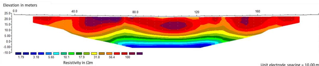
Figure 8. The 2D-resistivity profile contour obtained from inversion modeling on WP-04 trajectory
