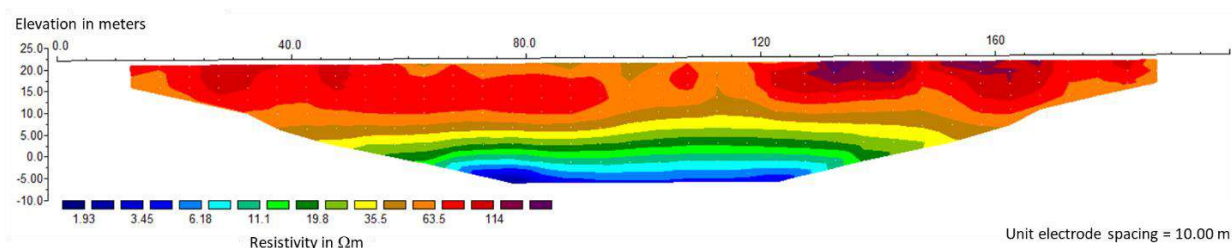
Figure 5. The 2D-resistivity profile contour obtained from inversion modeling on WP-01 trajectory
