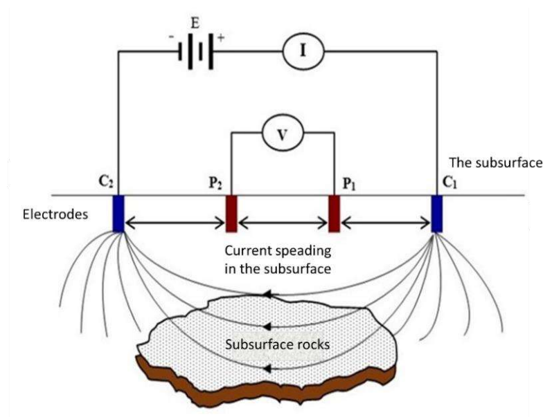
Figure 1. The scheme of 2D-resistivity data acquisition in the field
