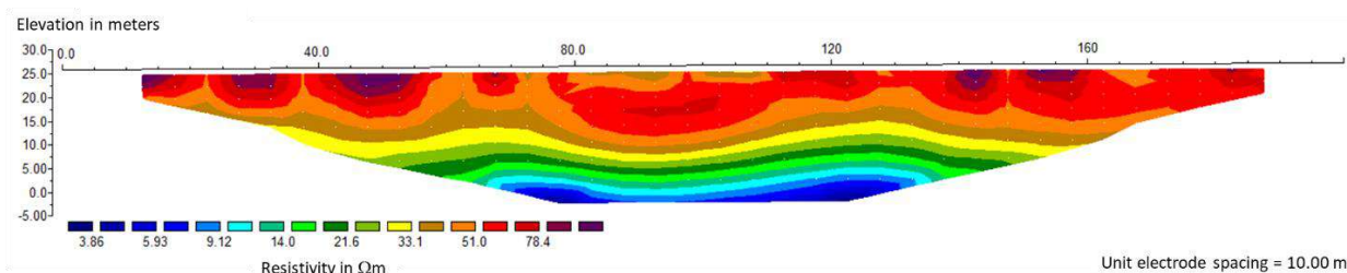
Figure 7. The 2D-resistivity profile contour obtained from inversion modeling on WP-03 trajectory
