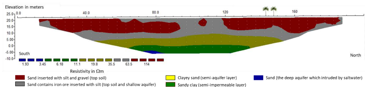
Figure 10. The 2D-hydrogeological profile contour of sub-surface rocks on the WP-01 trajectory
