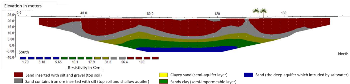
Figure 13. The 2D-hydrogeological profile contour of sub-surface rocks on the WP-04 trajectory
