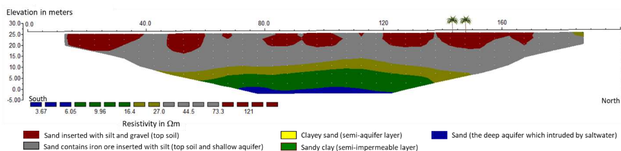
Figure 11. The 2D-hydrogeological profile contour of sub-surface rocks on the WP-02 trajectory
