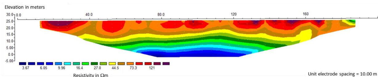
Figure 6. The 2D-resistivity profile contour obtained from inversion modeling on WP-02 trajectory
