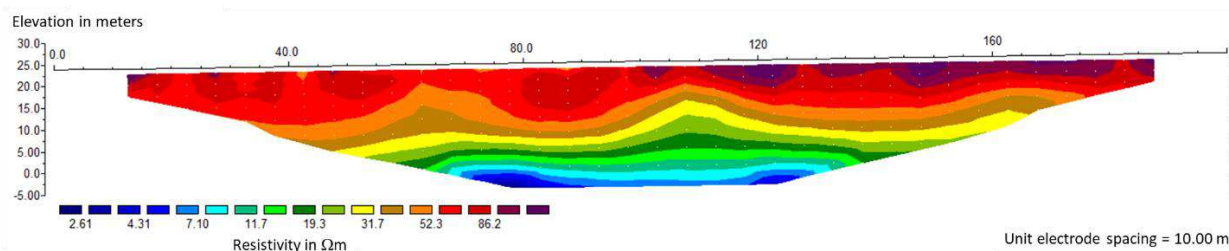
Figure 9. The 2D-resistivity profile contour obtained from inversion modeling on WP-05 trajectory
