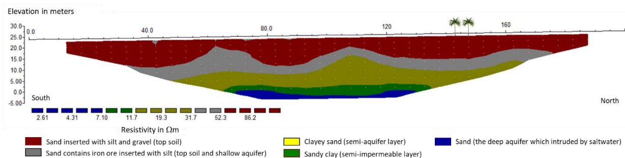
Figure 14. The 2D-hydrogeological profile contour of sub-surface rocks on the WP-05 trajectory
