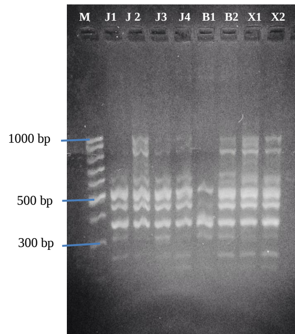
Fig. 4. PCR-RAPD using primer OPP-08 (M= DNA Ladder; J1= male 1; J2= male 2; J3= male 3; J4= male 4; B1= female 1; B2= female 2; X1= unknown sex 1; X2= unknown sex 2).
