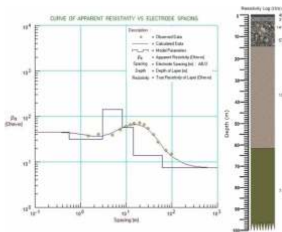
Figure 11. Resistivity curve and log at point Sch-5.
