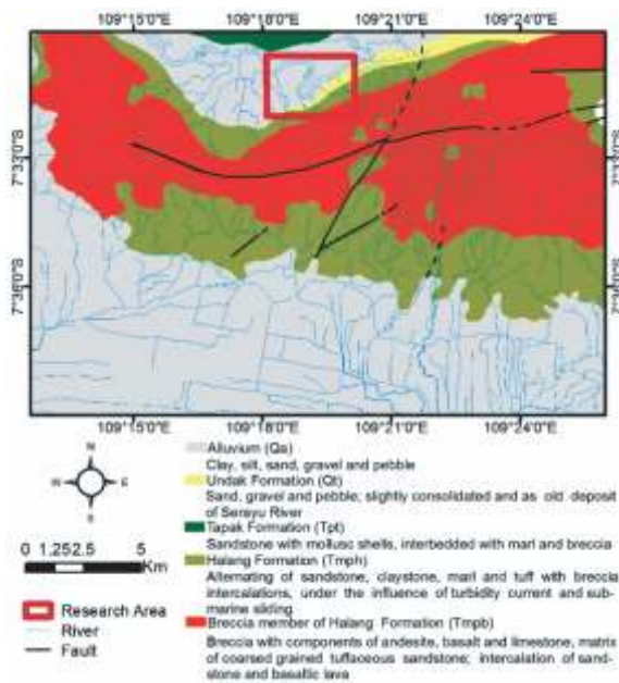
Figure 3. The geological map of the research area.
