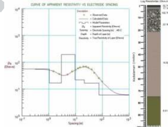
Figure 13. Resistivity curve and log at point of Sch-7.
