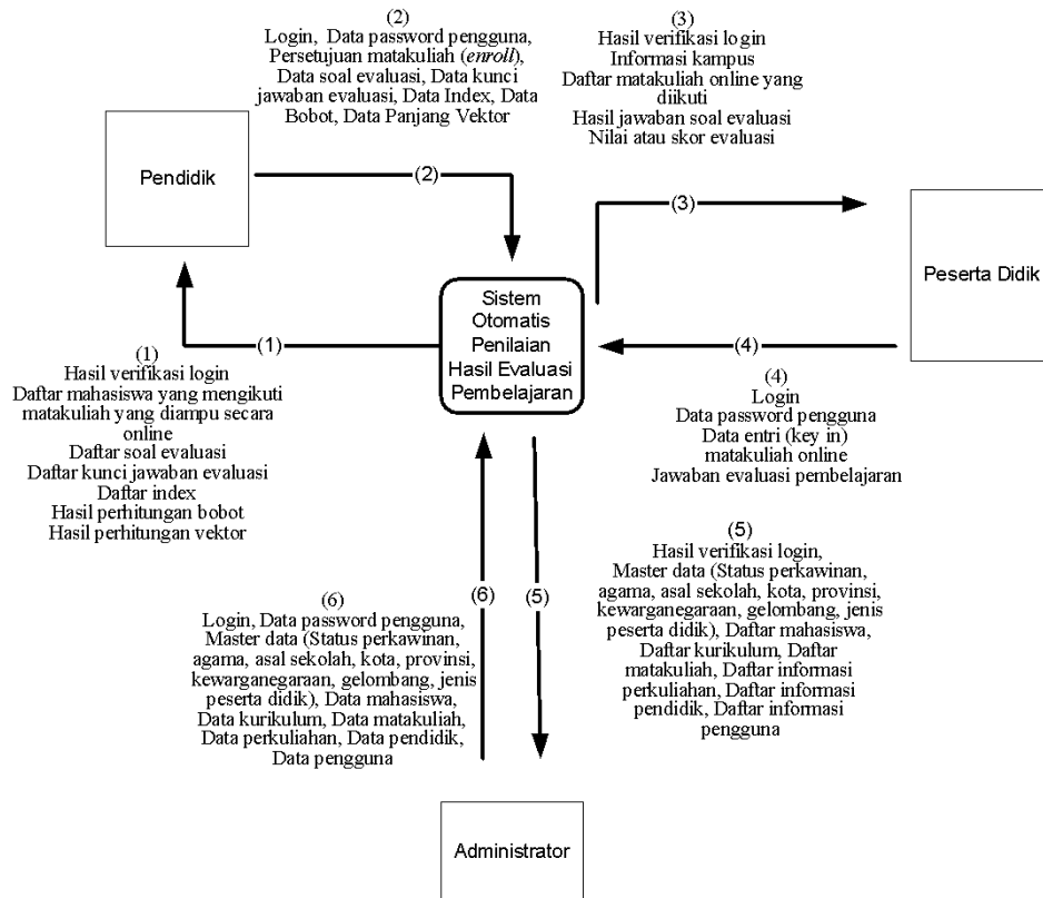
Gambar 2. DFD level 0
