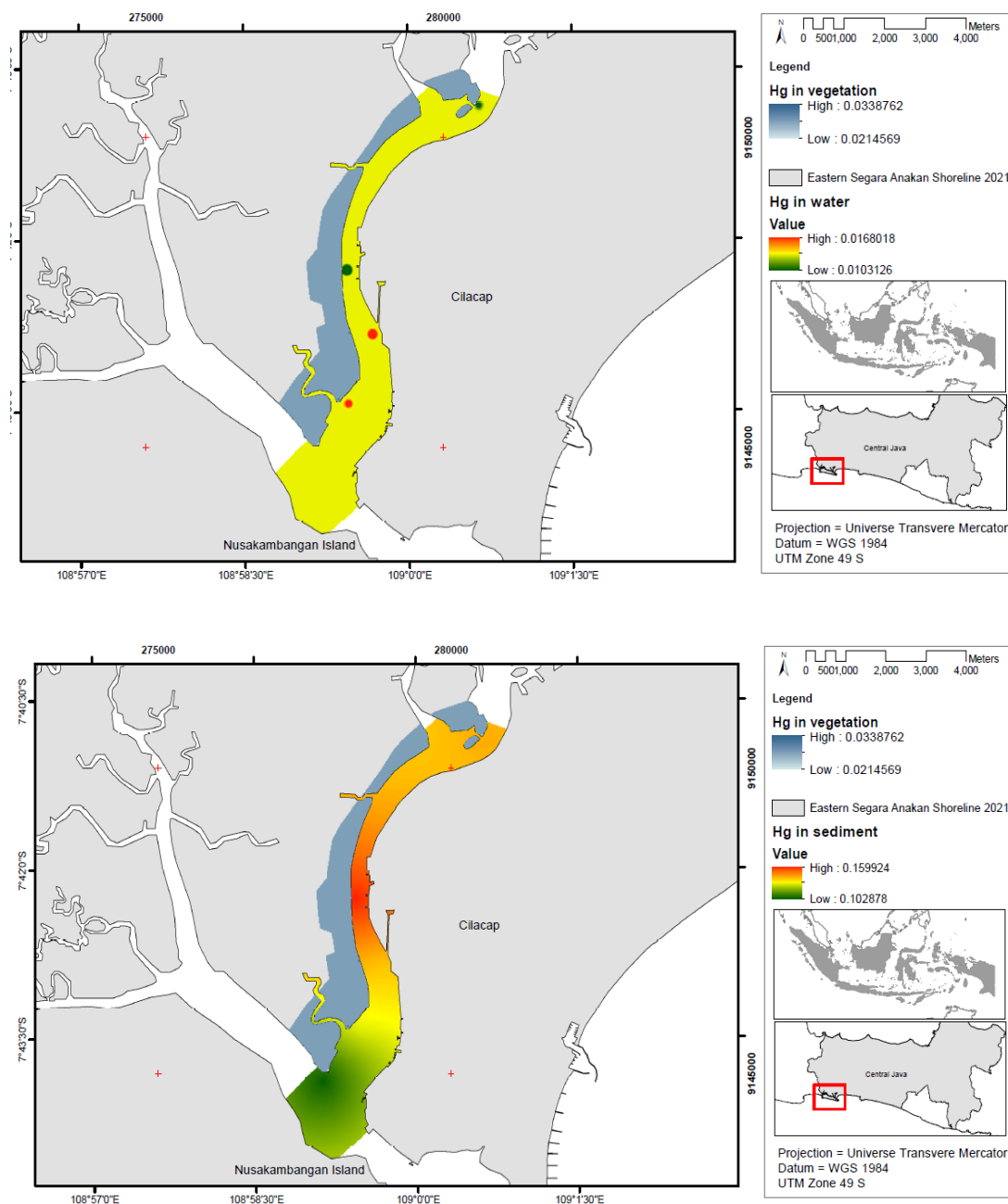
Figure 5. Interpolation of heavy metal contaminant distribution
