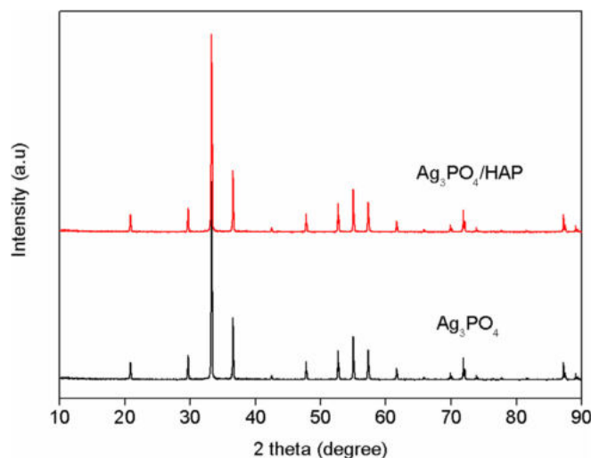
Fig. 1. XRD profile of \text{Ag}_3\text{PO}_4 (synthesized using \text{KH}_2\text{PO}_4 ) and \text{Ag}_3\text{PO}_4 /HAP (synthesized using hydroxyapatite).
