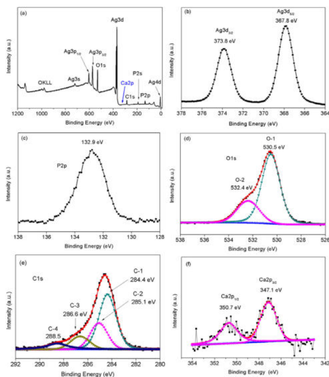
Fig. 4. XPS survey (a), \text{Ag}3d (b), P2p(c), O1s (d), C1s (e), and Ca2p (f) of \text{Ag}_3\text{PO}_4/\text{HAP} sample prepared by hydroxyapatite before photocatalytic reaction.
