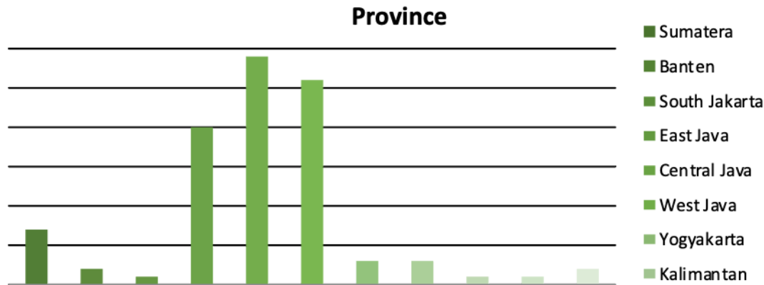
Graph 1. Distribution of Takaful Polis holders
