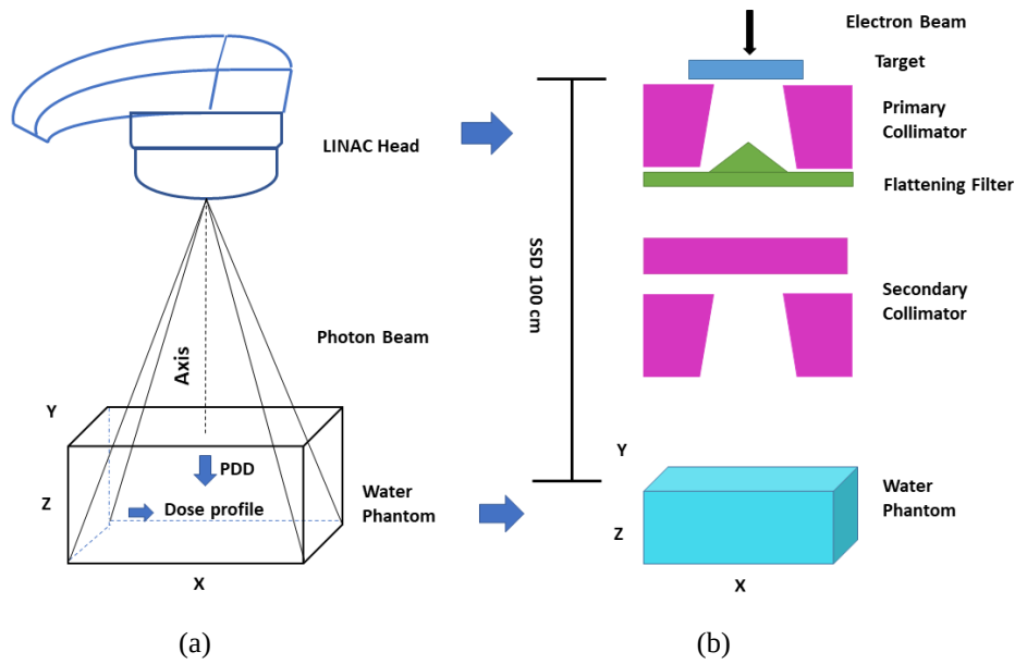
Fig. 2. (a) Geometry of Linac head and water phantom. The x-ray photon beam emitted from the LINAC head is applied to the water phantom. PDD measurement in the direction of the Z-axis and the dose profile perpendicular to the direction of the beam (in the direction of the X-axis), (b) Model of the LINAC head and visualization of the components that make up the LINAC head based on the Simen Primus device
