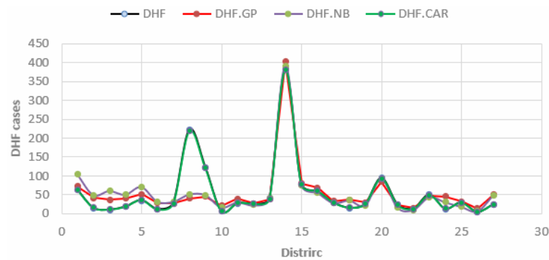
Figure 2. Plot of DHF actual and DHF predictions.
