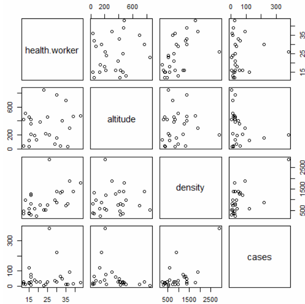
Figure 1. The scatterplot among variables.
