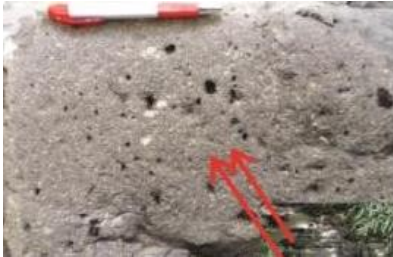
Figure 6. The appearance of basalt igneous rock in the study area [7].
