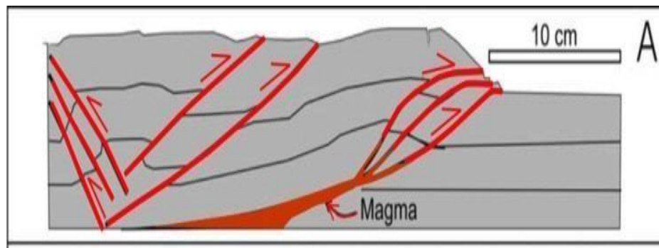
Figure 7. Intrusion models in contractional tectonic settings [24]. Shows the movement of magma under the surface along the plane of the thrust fault.
