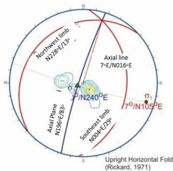
Figure 4. Stereographic analysis of Nanggulan folds.
