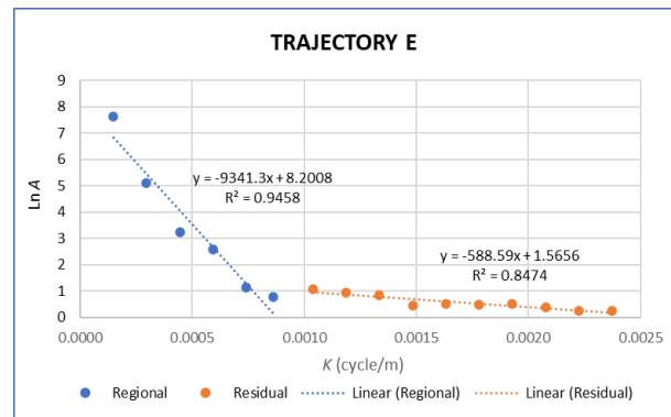
Figure 12. The result of power spectrum analysis of the CBA data on trajectory E which have been spread on a horizontal surface
