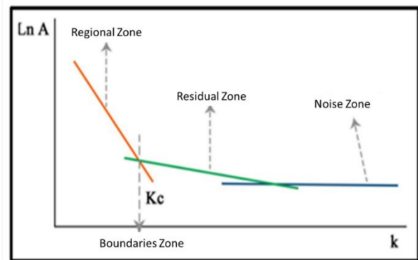
Figure 2 Linear regression procedure for spectrum analysis to estimate the maximum depth of regional and residual anomalous sources.
