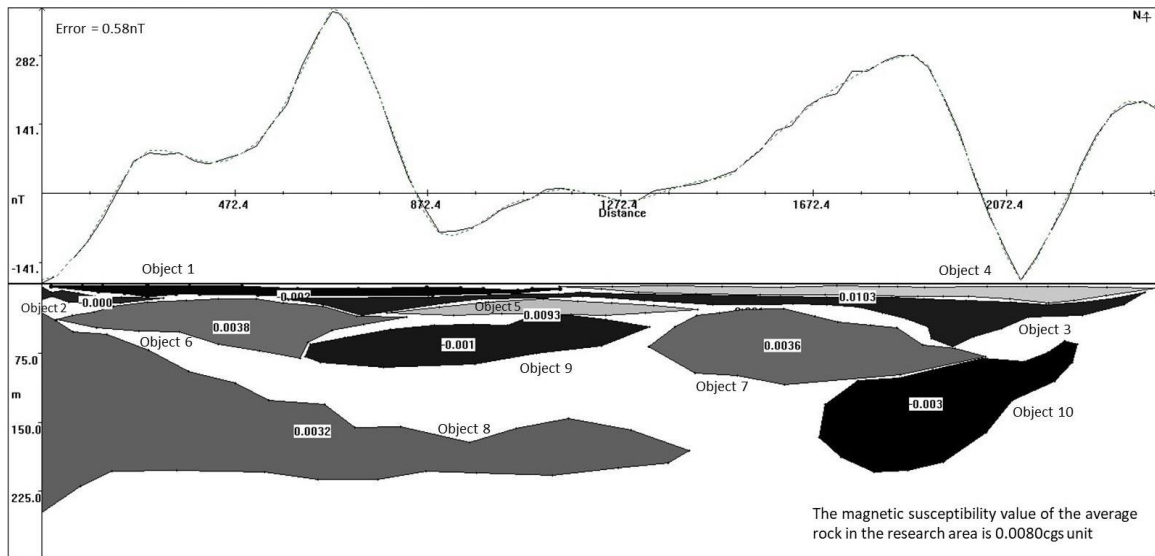
Figure 6. The modeling result using Mag2DC for Windows software on the magnetic anomaly data along the trajectory of AB and its interpretation (equipped the magnetic susceptibility contrast value of each model object).
