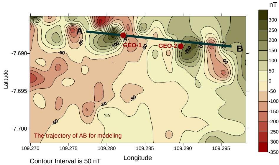
Figure 5. The contour map of local magnetic anomaly in the research area and the trajectory of AB for modeling. (Geo-1 and Geo-2 are locations of geoelectric sounding points in the research area)
