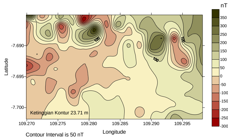
Figure 4. The contour map of the total magnetic anomaly distributed over the horizontal surface in the research area.
