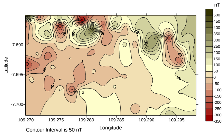
Figure 3. The contour map of the total magnetic anomaly distributed over the topographic surface in the research area
