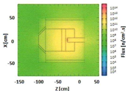
Figure 4 Distribution of fast neutron flux
