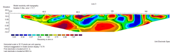
Gambar 9. Penampang resistivitas 2D Lintasan Wen3
