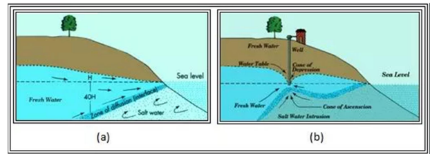
Gambar 3. (a) Keadaan interface alami, (b) Interface mengalami intrusi [14]
