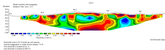
Gambar 8. Penampang resistivitas 2D Lintasan Wen2
