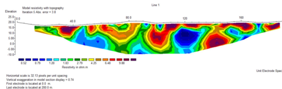
Gambar 7. Penampang resistivitas 2D Lintasan Wen1
