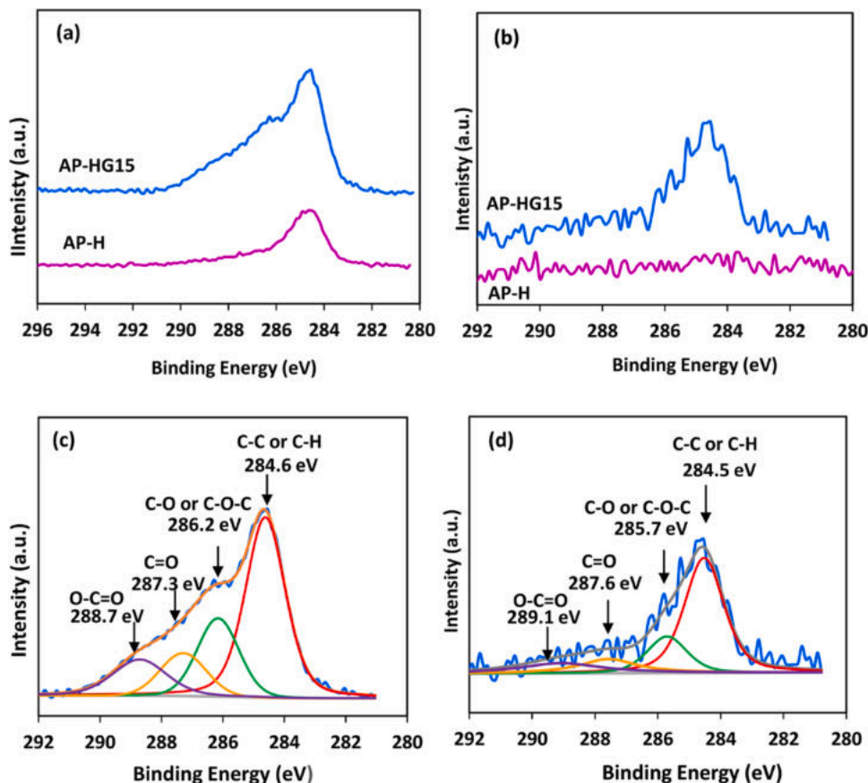
Fig. 8. C1s XPS of AP-H and AP-HG15 (a), C1s after \text{Ar}^+ sputtering treatment (b), and C1s deconvolution of AP-HG15 (c) and after \text{Ar}^+ sputtering treatment (d).
