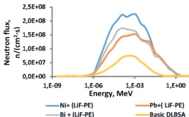
Fig. 2. The neutron flux spectrum of DLBSA output without and with nozzles. (See color Figure on the journal website.)
