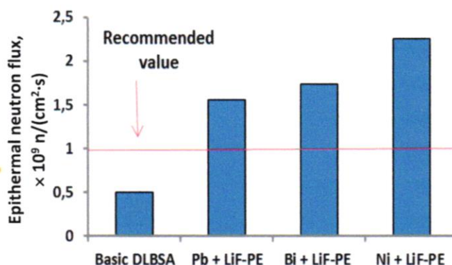
Fig. 3. The comparison of epithermal neutron flux of DLBSA output without and with nozzles. (See color Figure on the journal website.)
