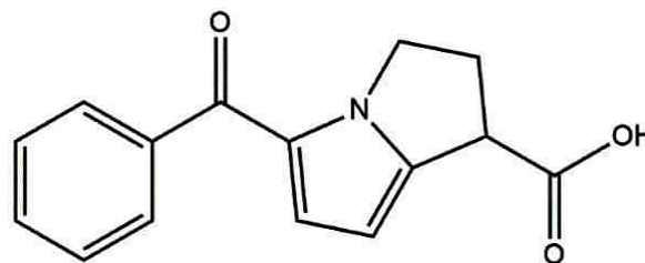
Figure 1. Chemical structure of ketorolac
