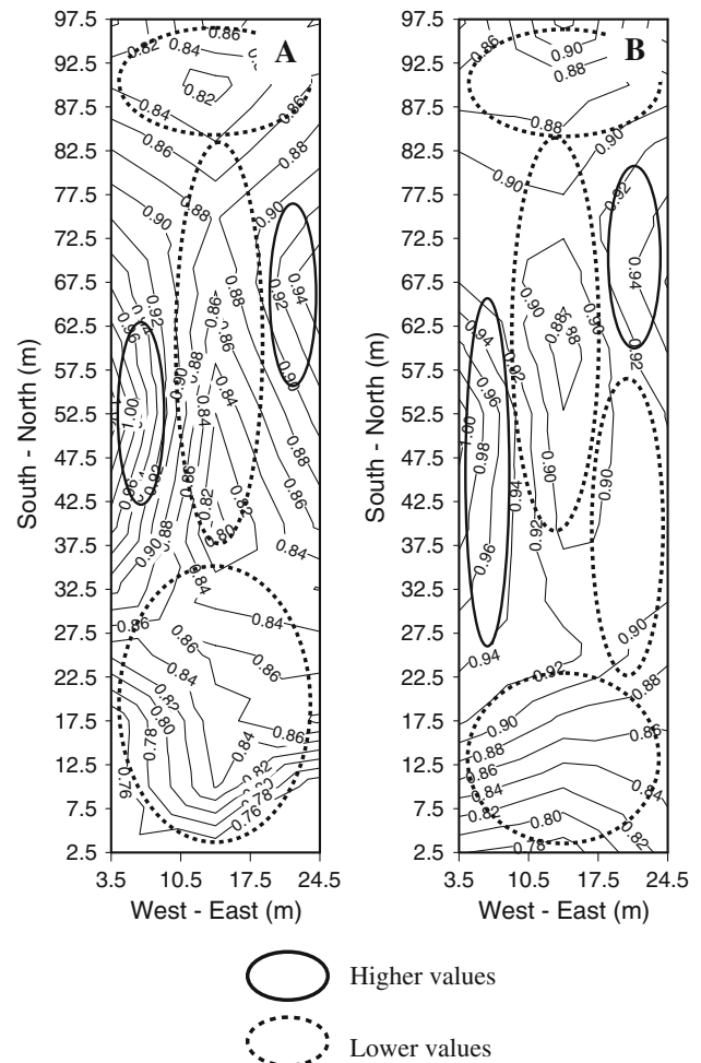
Fig. 5 Contour map of: predicted (a) and measured \rho_b (b)
