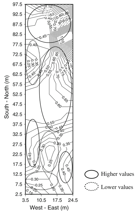
Fig. 7 Contour map of subsurface percolation rate
