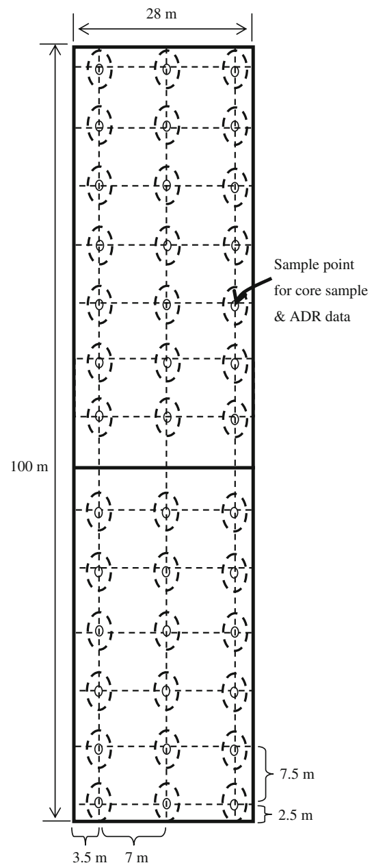
Fig. 1 Experimental plot of Fuchu Honmachi paddy field
