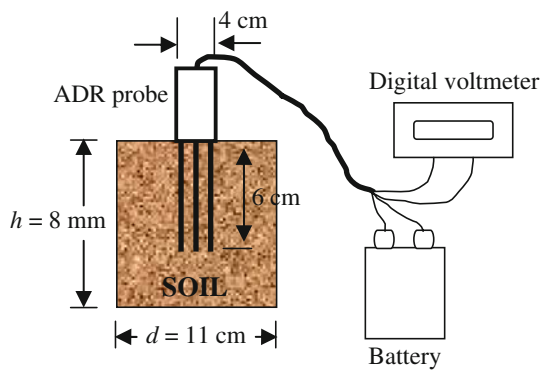
Fig. 2 Calibration of ADR probe
