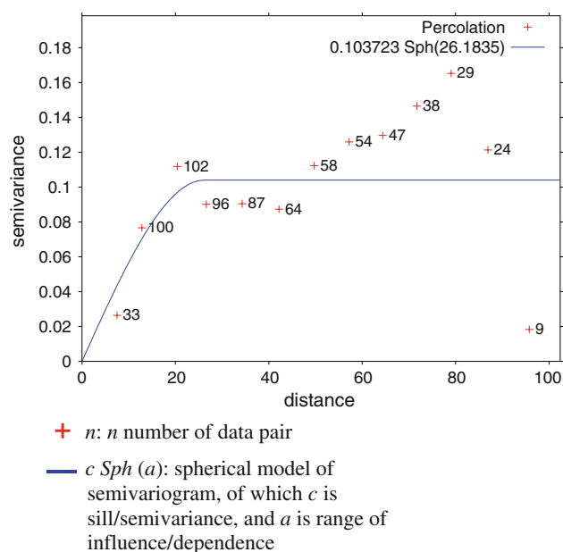
Fig. 10 Semivariogram of subsurface percolation rate
