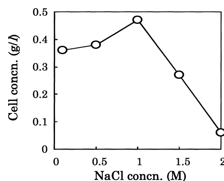
FIG. 1. Effect of initial NaCl concentration on cell growth. Test tube cultivations were performed with several initial NaCl concentrations. The average of duplicate cultivations was shown.
