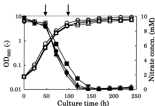
FIG. 3. Addition of NaCl during the culture with initial NaCl concentration of 1.0 M. During cultivation in Roux bottle with initial NaCl concentration of 1.0 M, NaCl was added at mid-log phase (triangles, 0.5 M) or the end of log phase (reverse triangles, 0.5 M; squares, 1.0 M). The data without NaCl addition during the culture was shown with circles. The addition times are indicated by arrows. OD 680 (open symbols) and nitrate concentration (closed symbols) were measured. The average of duplicate cultures was shown.
