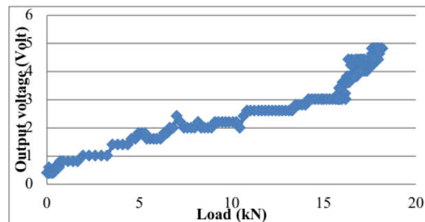
FIGURE 11. F Relationship between test load and output voltage failure detection system for Beam 2
