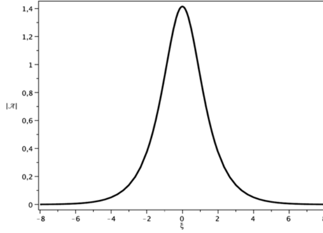
Figure 3. Bright soliton for \gamma = 1 and \beta = 1 .
