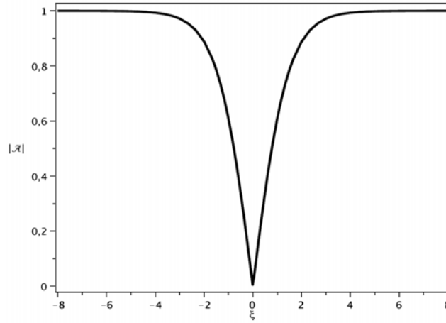
Figure 2. Dark soliton for \gamma = -1 and \beta = 1 .
