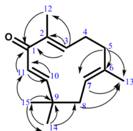
Figure 2. HMBC of zerumbone
