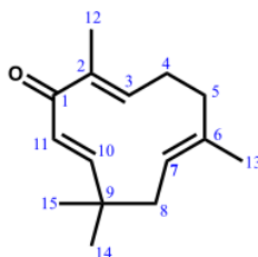
Figure 1. Zerumbone
