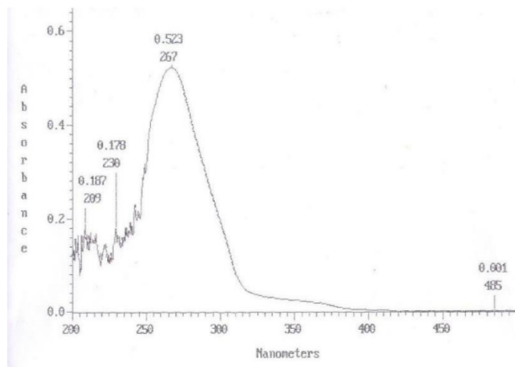
Figure 2. The UV-Visible spectrum of ethyl acetate fraction
